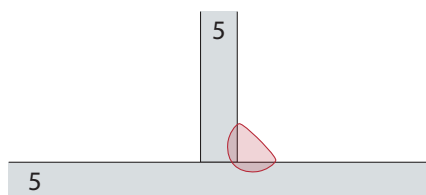
S355, tloušťka plechu 5 mm
